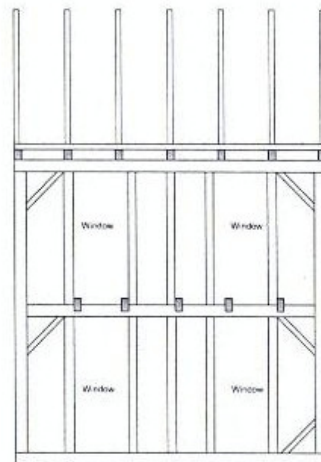
WALL Z
