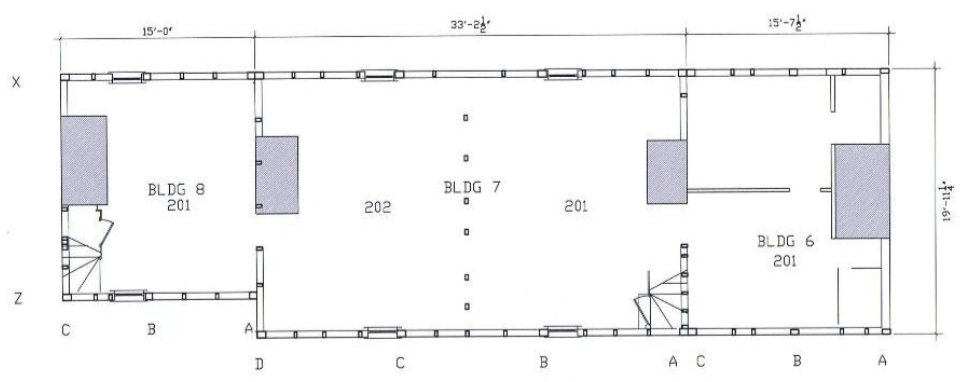
FIRST FLOOR PLAN Scale: 1/8"=1'-0" 1" 5' 10'
