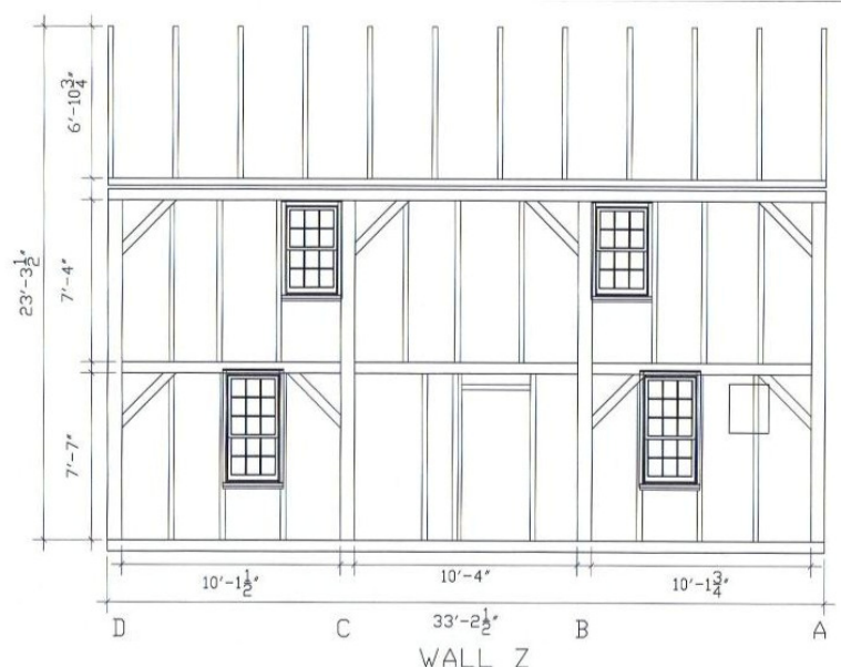
CENTER WING TIMBER FRAME Scale: 3/16"=1'-0" 1" 5' 10'
